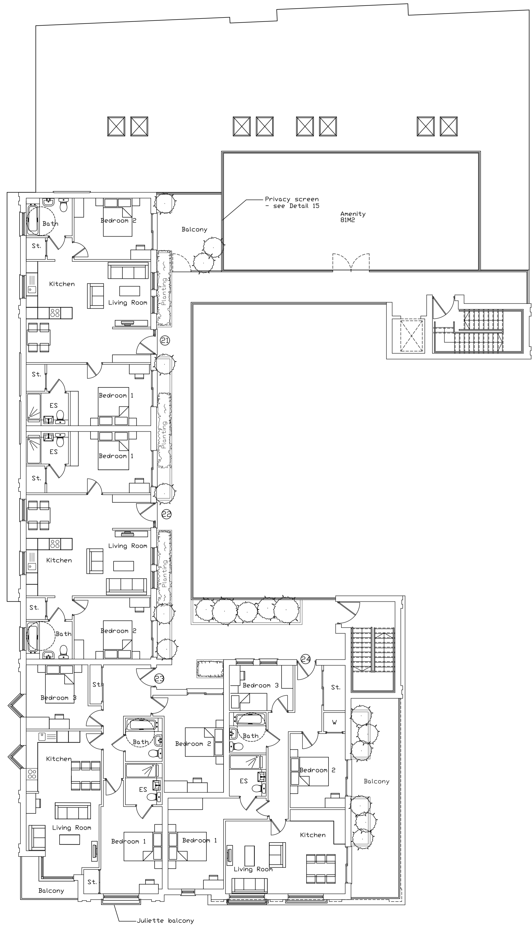
Proposed Third Floor Plan Scale 1:100 @ A1
